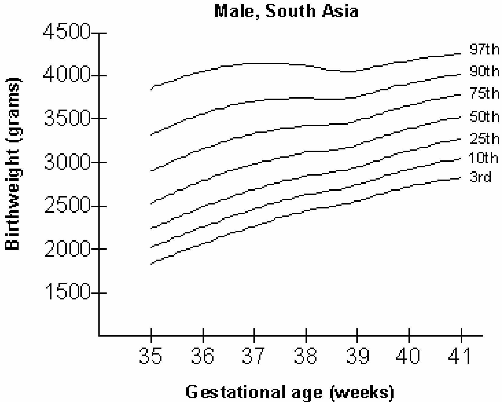
Smoothed birth weight centile curves for male singleton infants of South Asian maternal ancestry. (Source: JG Ray, D Jiang, M Sgro, R Shah, G Singh, M Mamdani)
